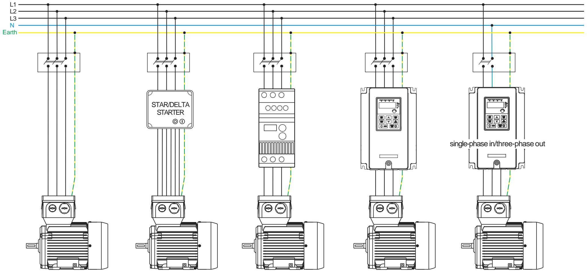
DOL (Direct On Line) Motor wound in STAR or DELTA for Mains Voltage
